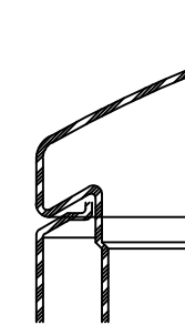
LIP DETAIL SCALE: 1 1/2" = 1'-0"
