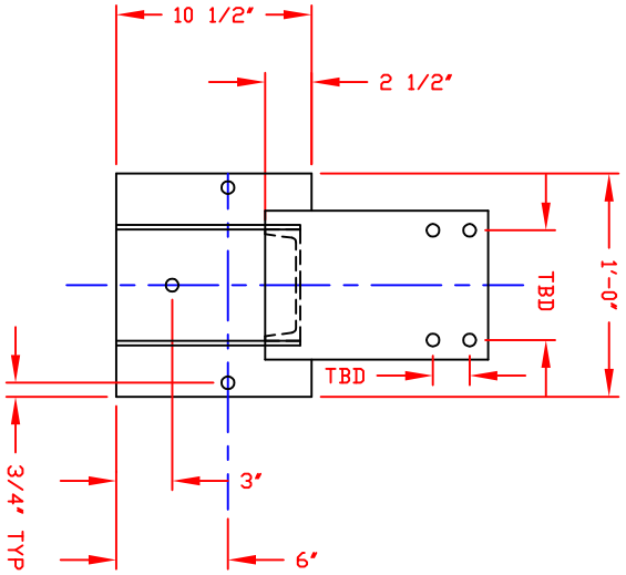
BASEPLATE DETAIL SHOWING CHANNEL & GUSSETS
