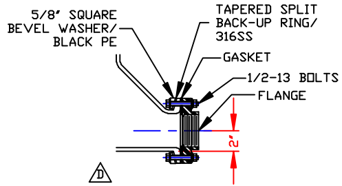
DETAIL "A" (INTEGRALLY MOLDED FLANGED OUTLET) AVAILABLE IN 3" SIZE ONLY SCALE: NONE
