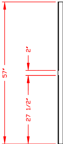
DETAIL ④ 1 1/2' X 1 1/2' X 3/16" ANGLE (2) REQ'D
