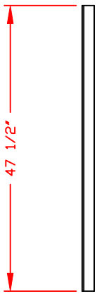
DETAIL ③ 2' X 2' X 1/4" ANGLE (4) REQ'D
