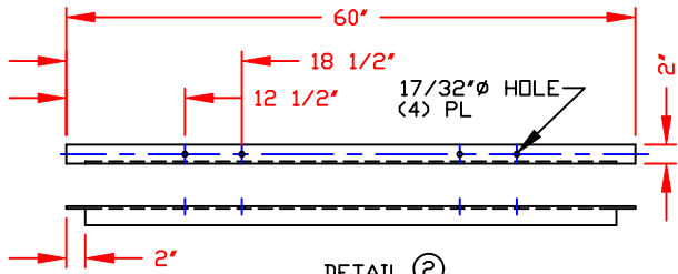
DETAIL ② 2' X 2' X 1/4' ANGLE (2) REQ'D
