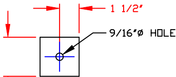
DETAIL ⑨ 1/4" THK PLATE (4) REQ'D SCALE: 3"=12"
