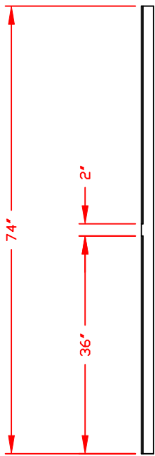
DETAIL ④ 1 1/2' X 1 1/2' X 1/4' ANGLE (2) REQ'D
